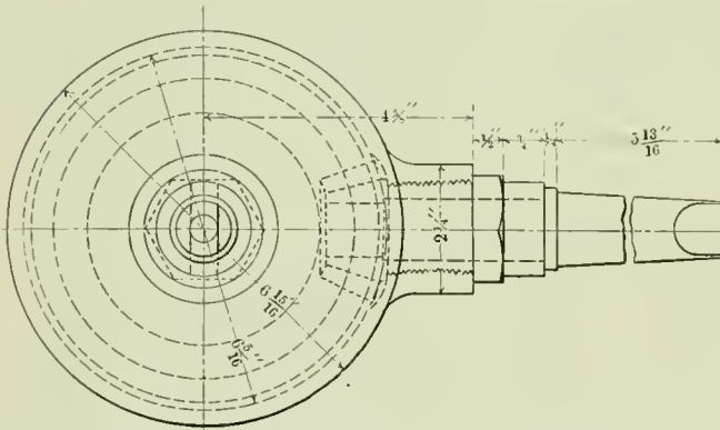
FIG. 2.—ANGLE DEVICE FOR DRILLING AND REAMING IN CLOSE QUARTERS. THREE SIZES ARE MADE, THE ILLUSTRATION SHOWING THE LARGEST.
